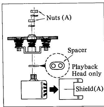
Fig. 6-1 Head Replacement
