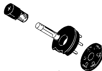
Fig. 7-7 Voltage Conversion
