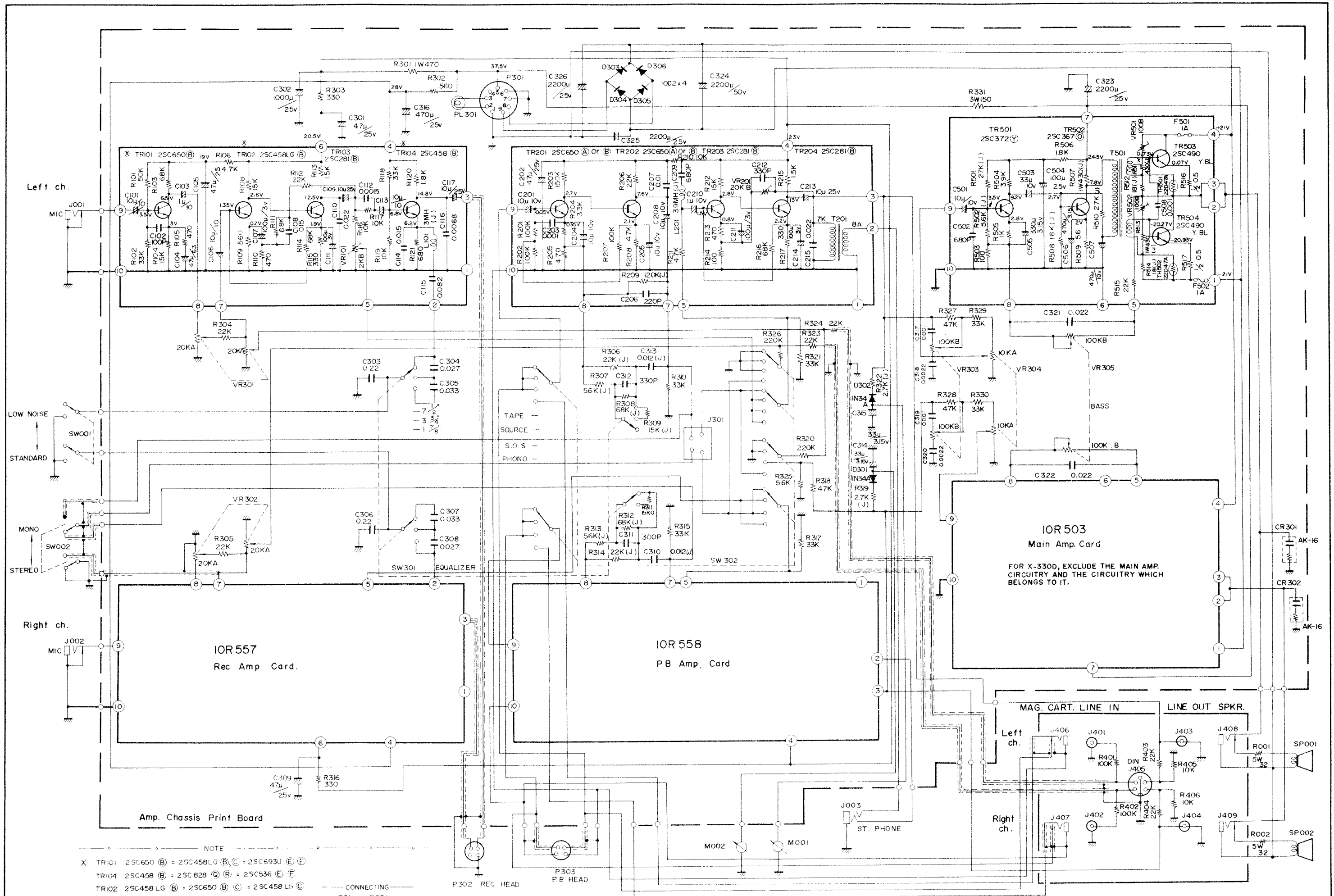
NO.2-2 X-330·X-330D AMP. SCHEMATIC DIAGRAM 13818563
