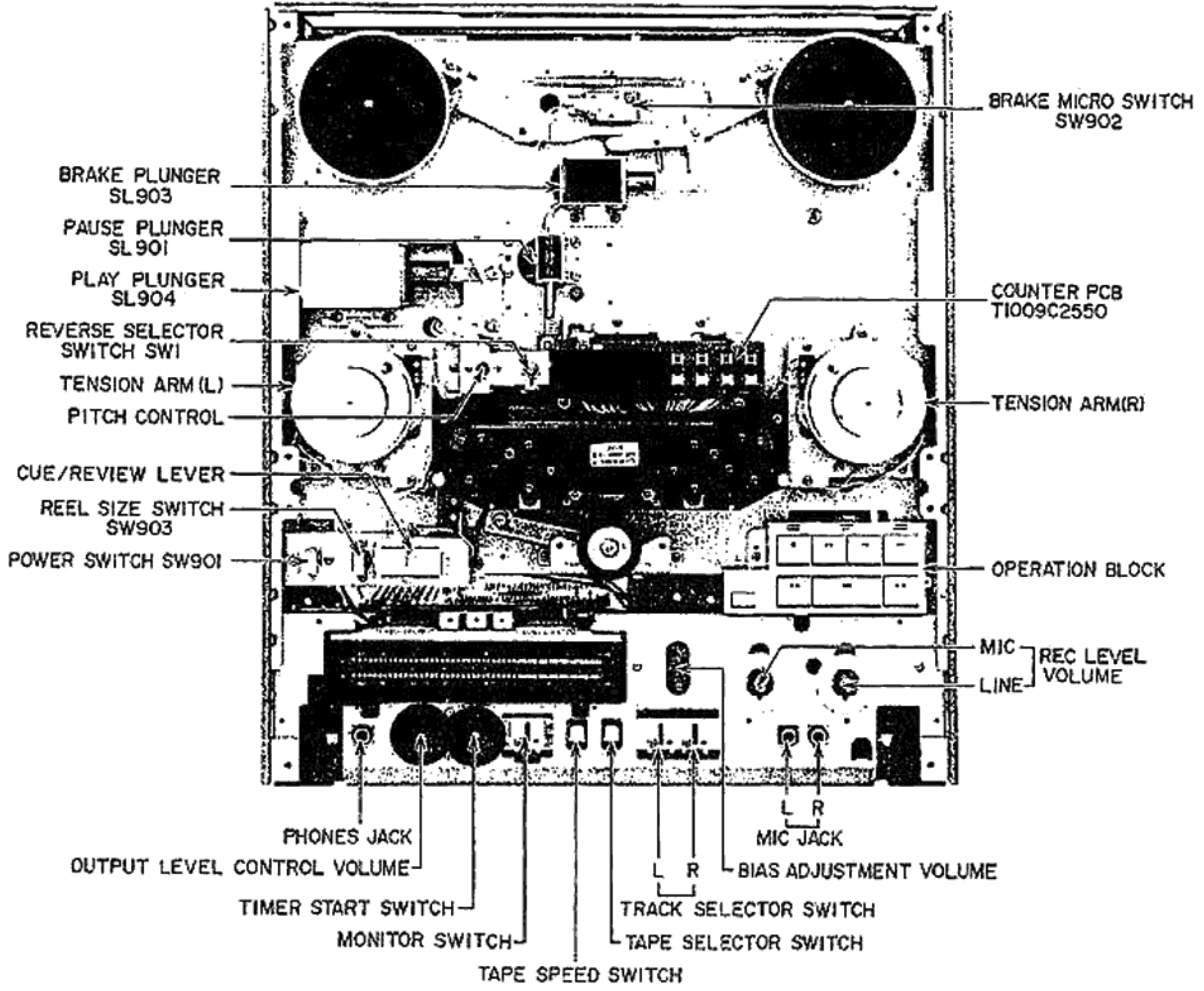
Fig. 2 Front View
