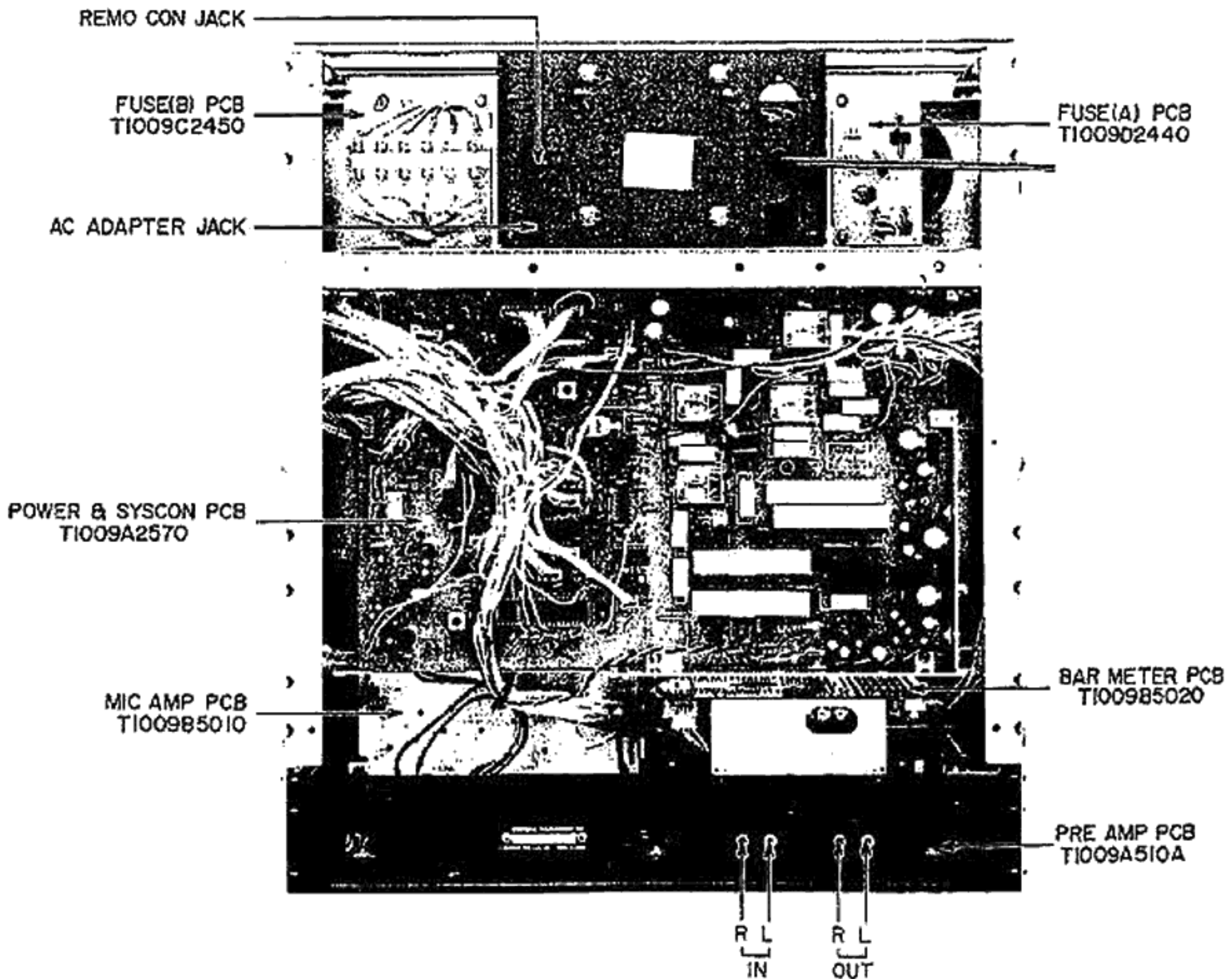
Fig. 3 Rear View
