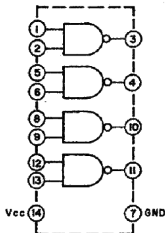
MC14011BCP
