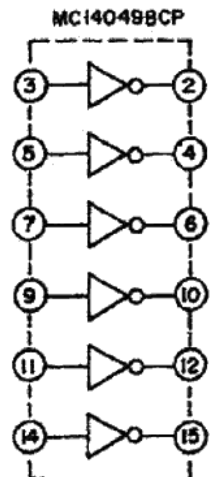
MC14049BPC
