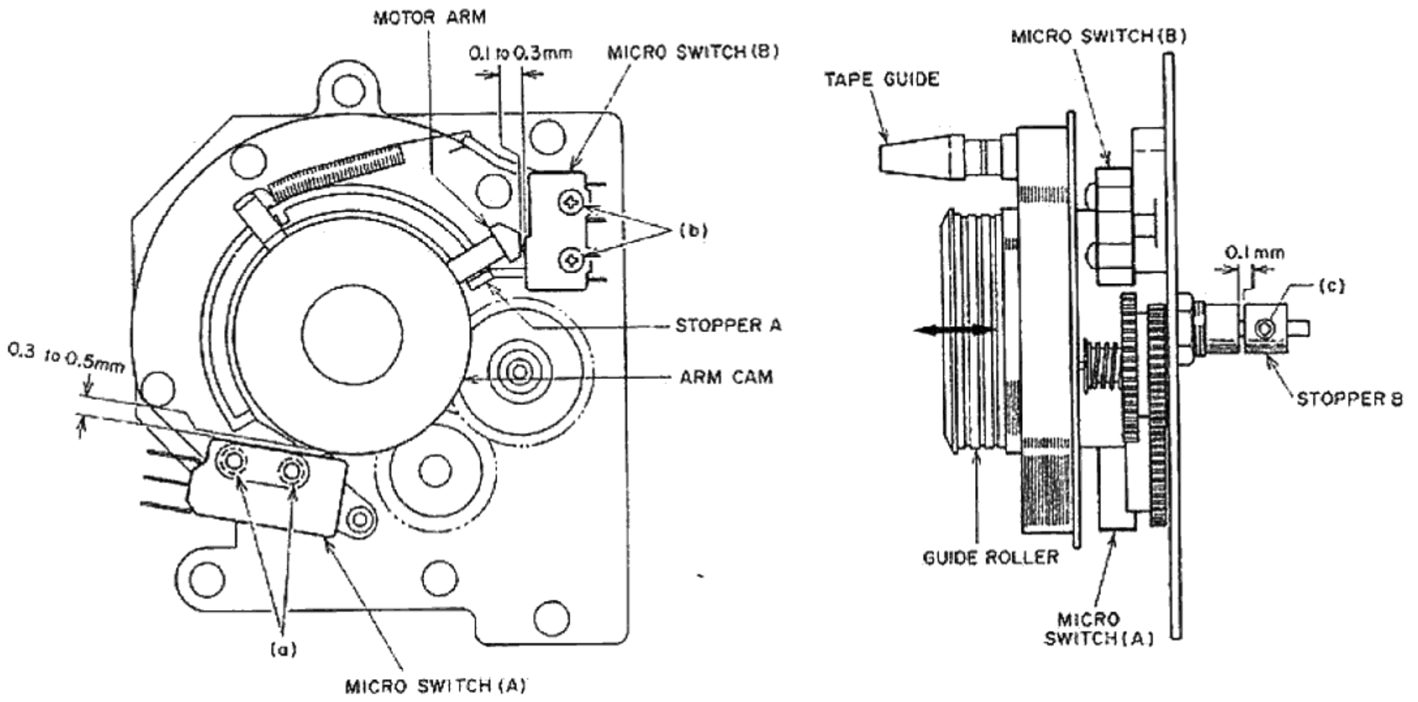
Fig. 33 Roller Block
