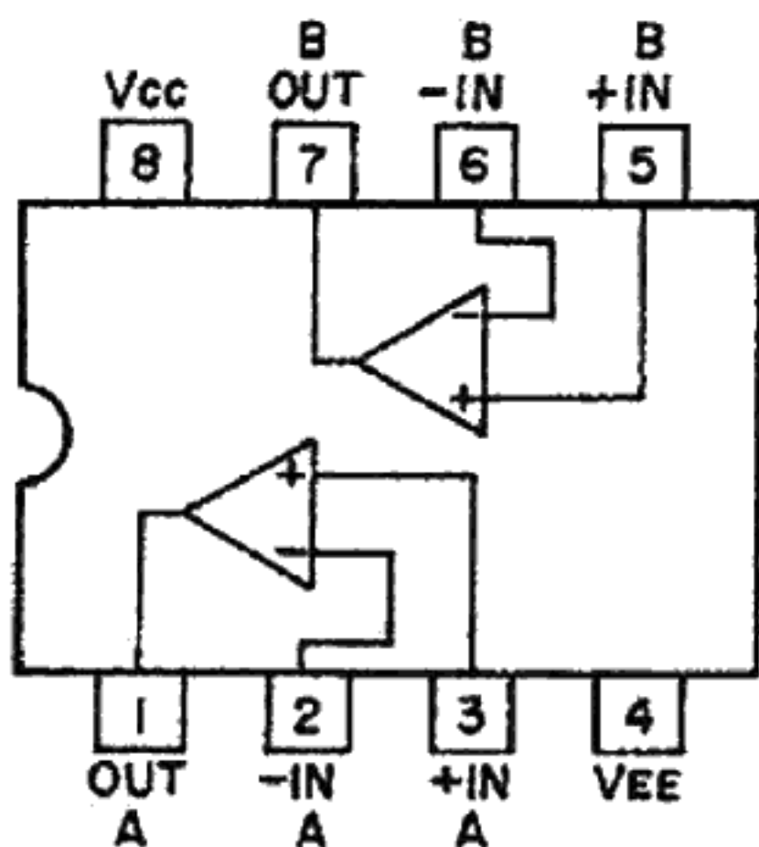
NJM4558D
