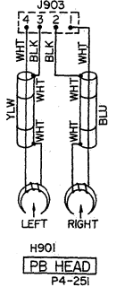
PRE AMP P.C BOARD TG-5001A
