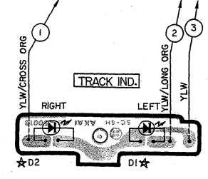
LED P.C BOARD TG-5001B
