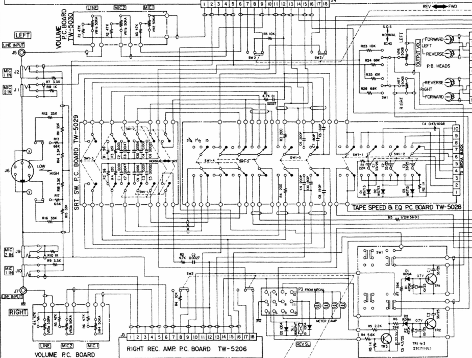
RIGHT REC. AMP. P.C. BOARD TW-5206
