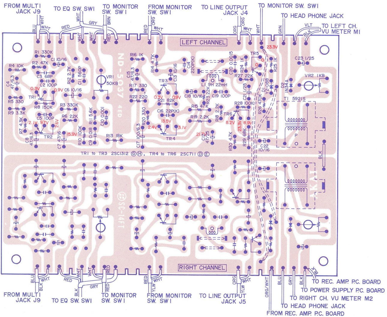
Fig. 23 PLAYBACK AMP. P.C. BOARD ND-5037 (Reverse Side)
