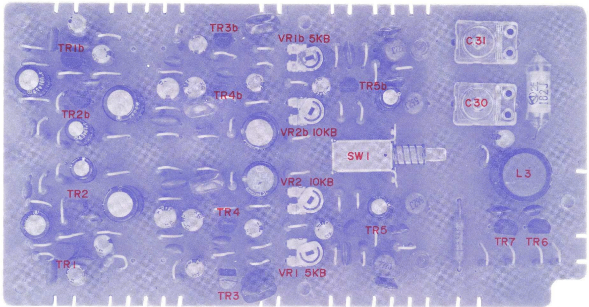
Fig. 24 RECORDING AMP. P.C. BOARD MU-5016
