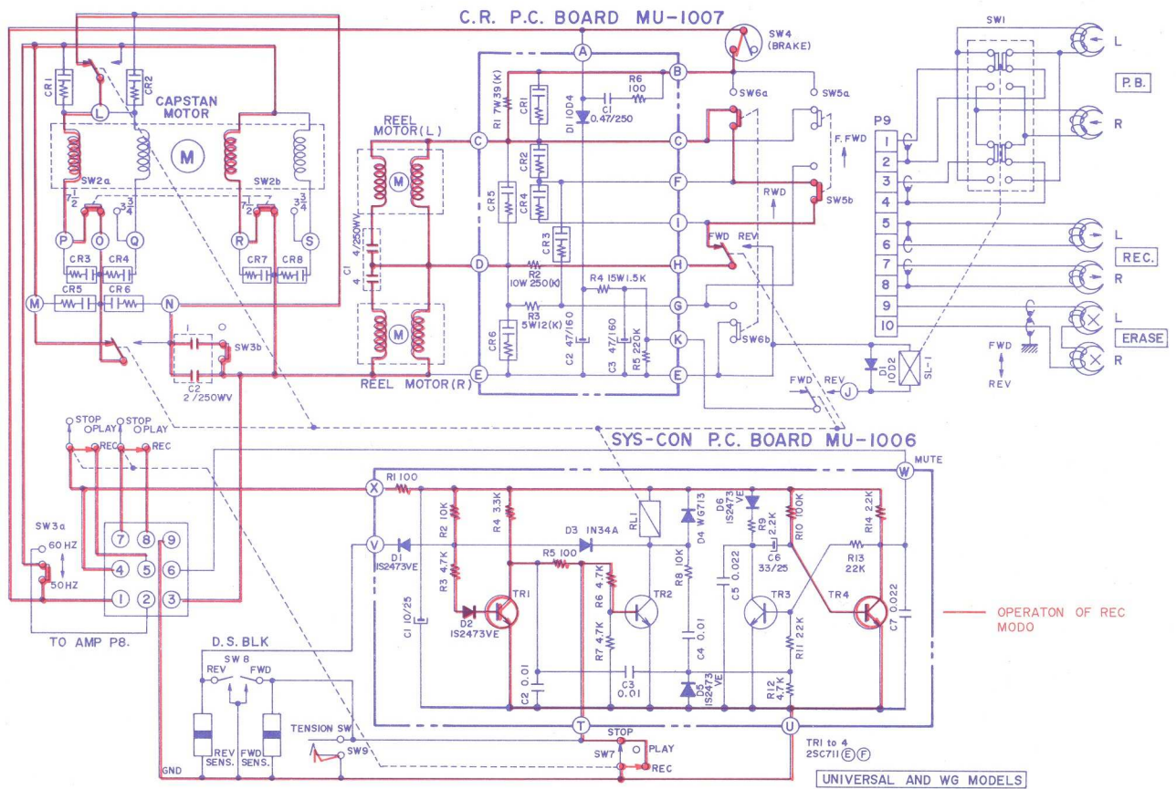
SCHMATIC 4
