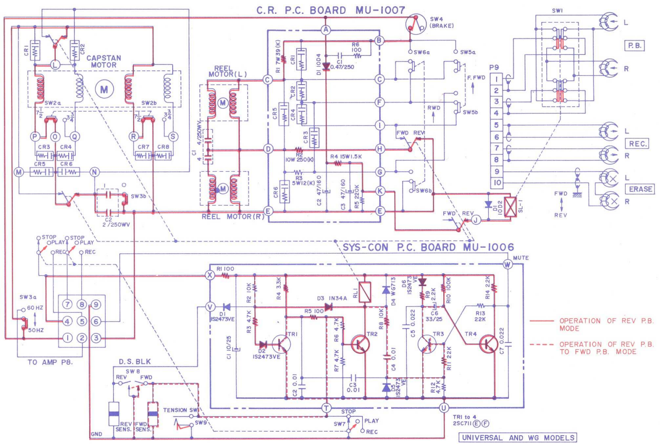
SCHMATIC 3
