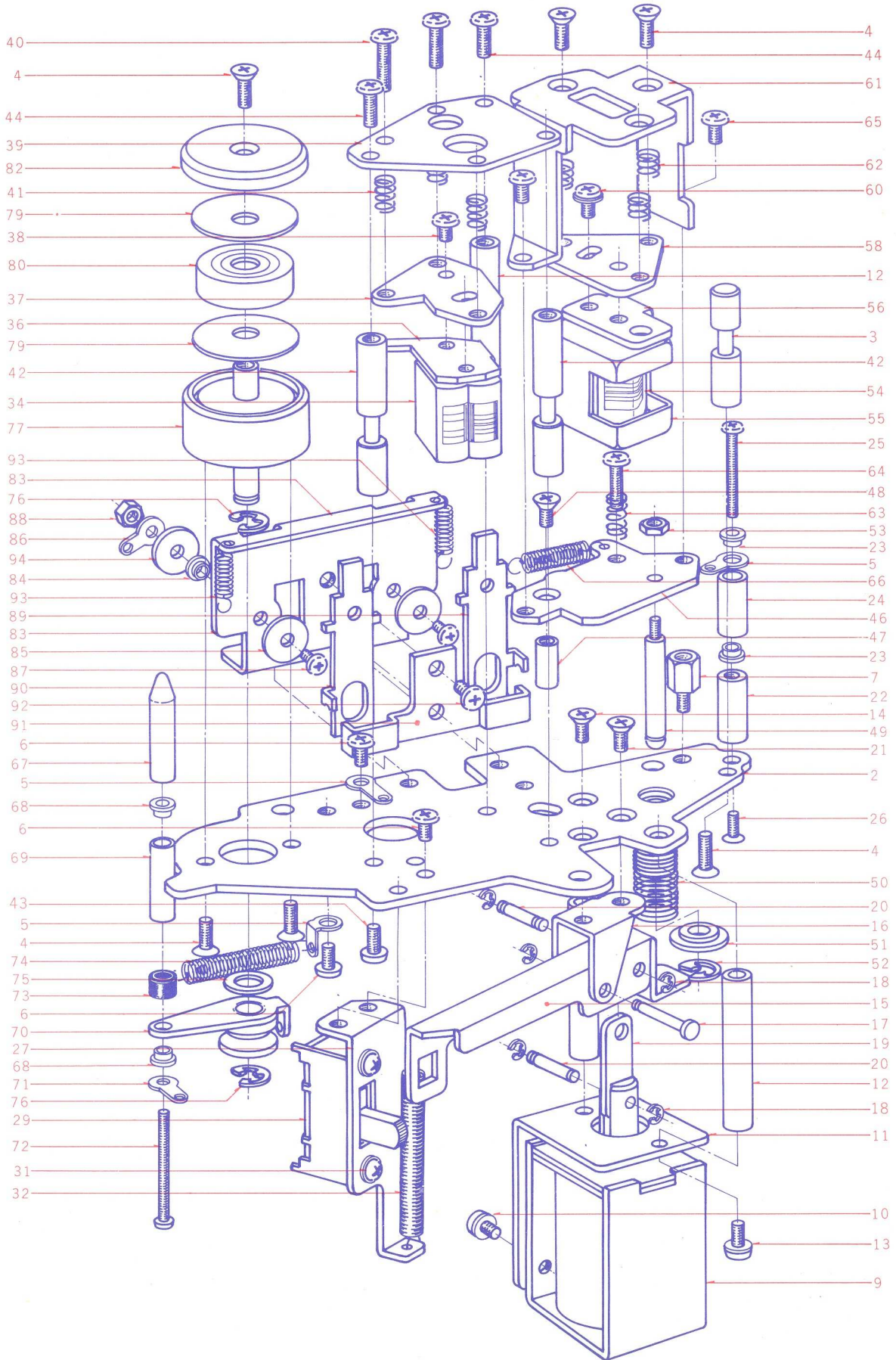
FIG. 1 ILLUSTRATION OF MU GX HEAD BLOCK
