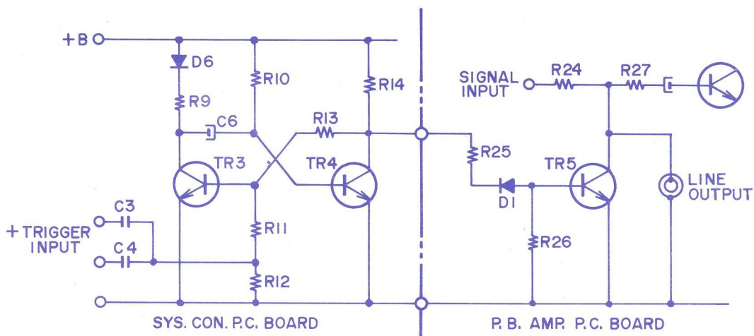
SCHEMATIC 7
