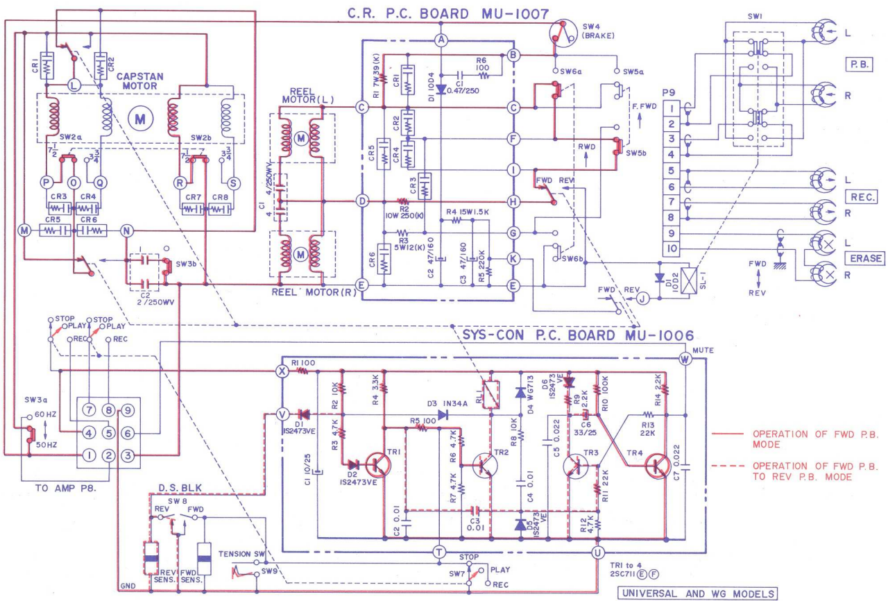
SCHMATIC 2
