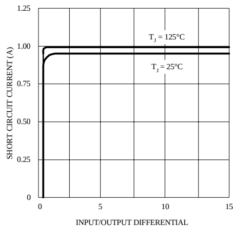
Short-Circuit Current
