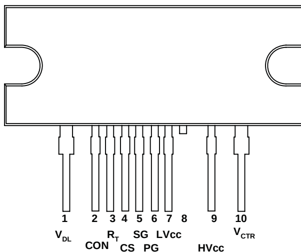
Figure 3. Package Diagram
