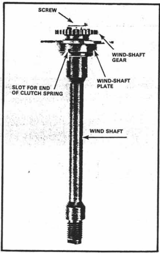
Figure 219 This is how you get a replacement wind-shaft assembly; you can't obtain individual replacement components.
