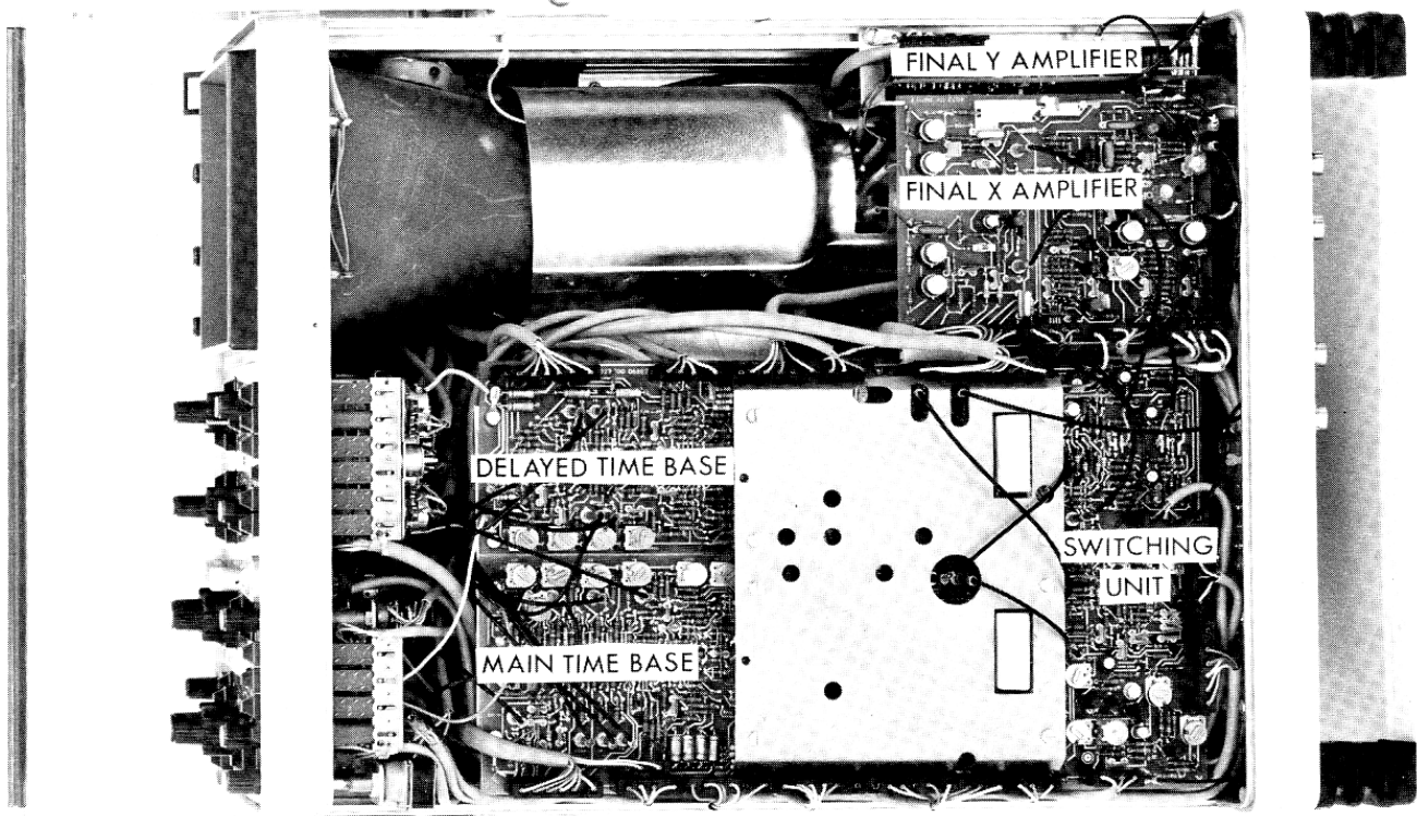
Fig. 3.25. Top view
