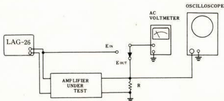
Fig. 2-1 Interconnections of the equipment.
