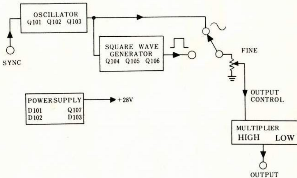
Fig. 3-1 Block diagram: LAG-26
