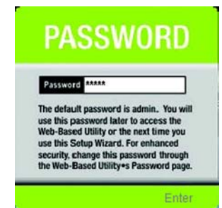
Figure 5-7: Password Screen
