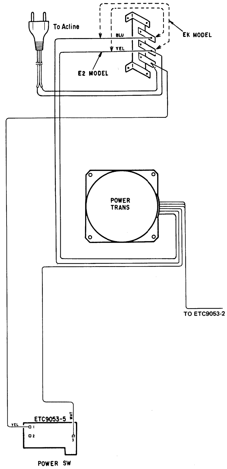
WIRING DIAGRAM E2 & EK Models (Same as EU version except the following)
