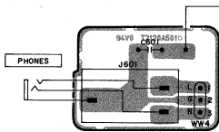
HEADPHONE PCB T2120A50ID
