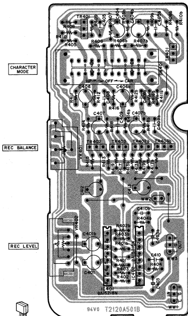
VOLUME PCB T2120A50IB
