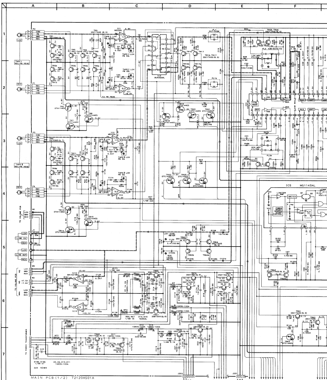
MAIN PCB (1/2) T2120A501A
