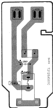
POWER SW PCB T2120A50IC
