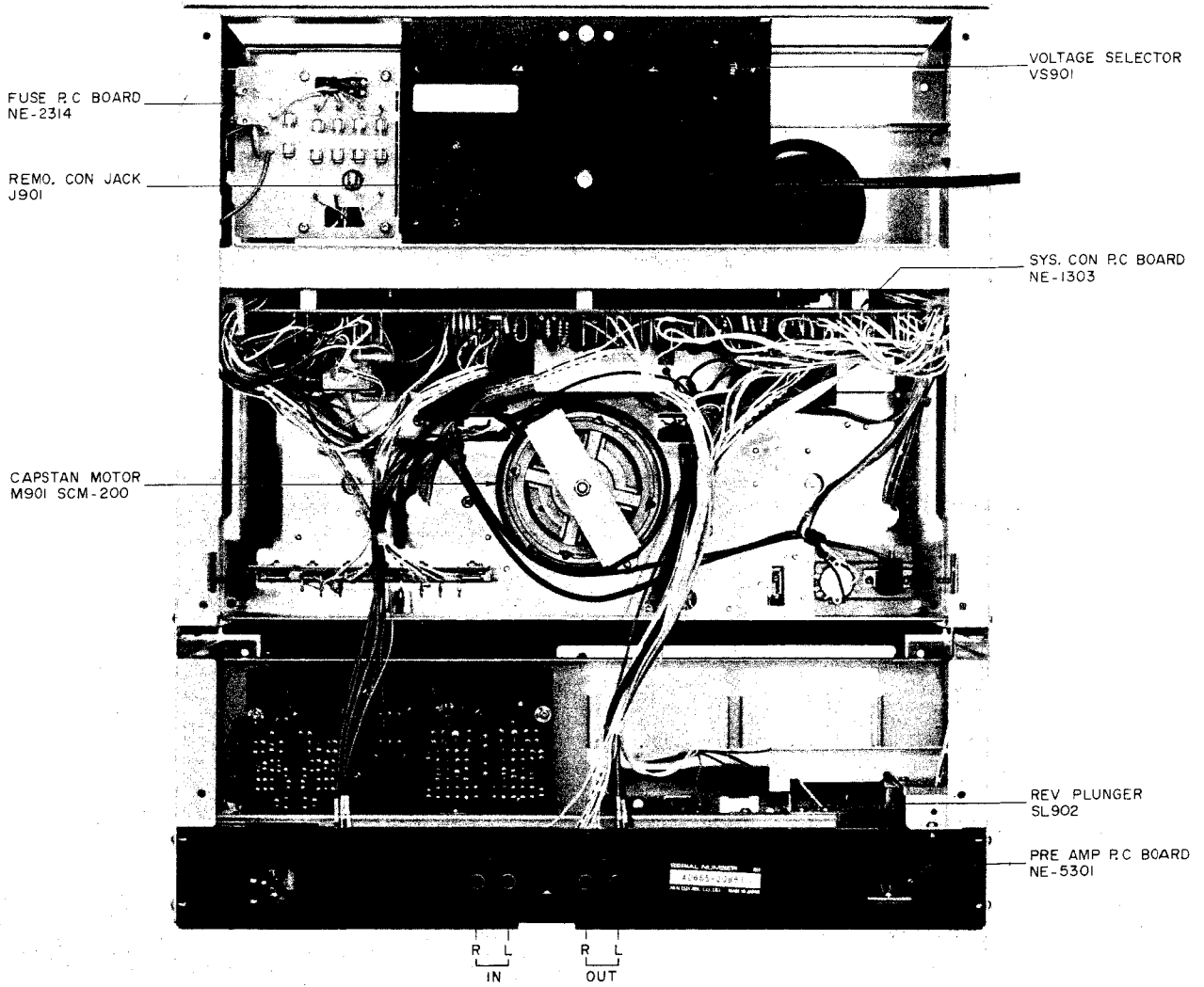
Fig. 3 Rear View
