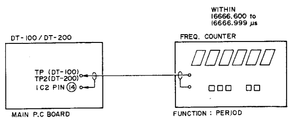
Fig. 7 Instrument Connections
