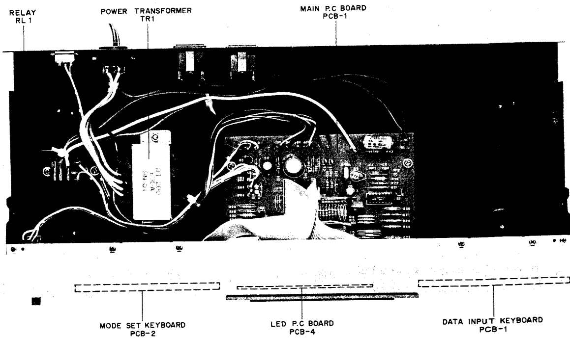
Fig. 4 Top View
