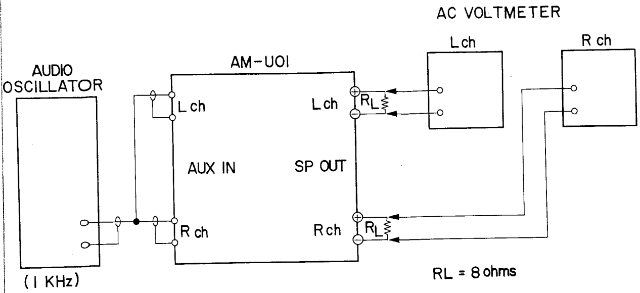
Fig. 5 Instrument Connections
