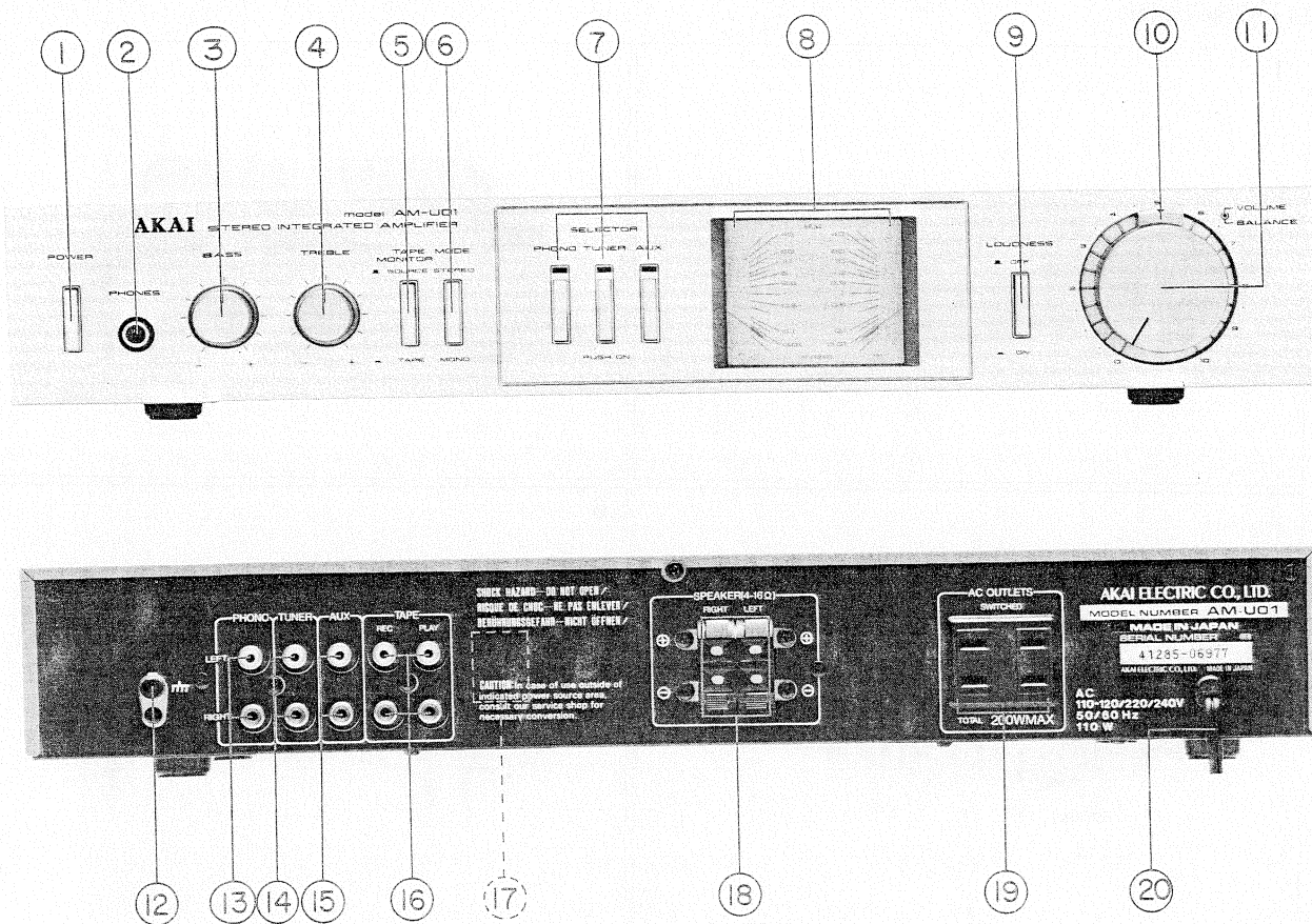
Fig. 1 Controls
