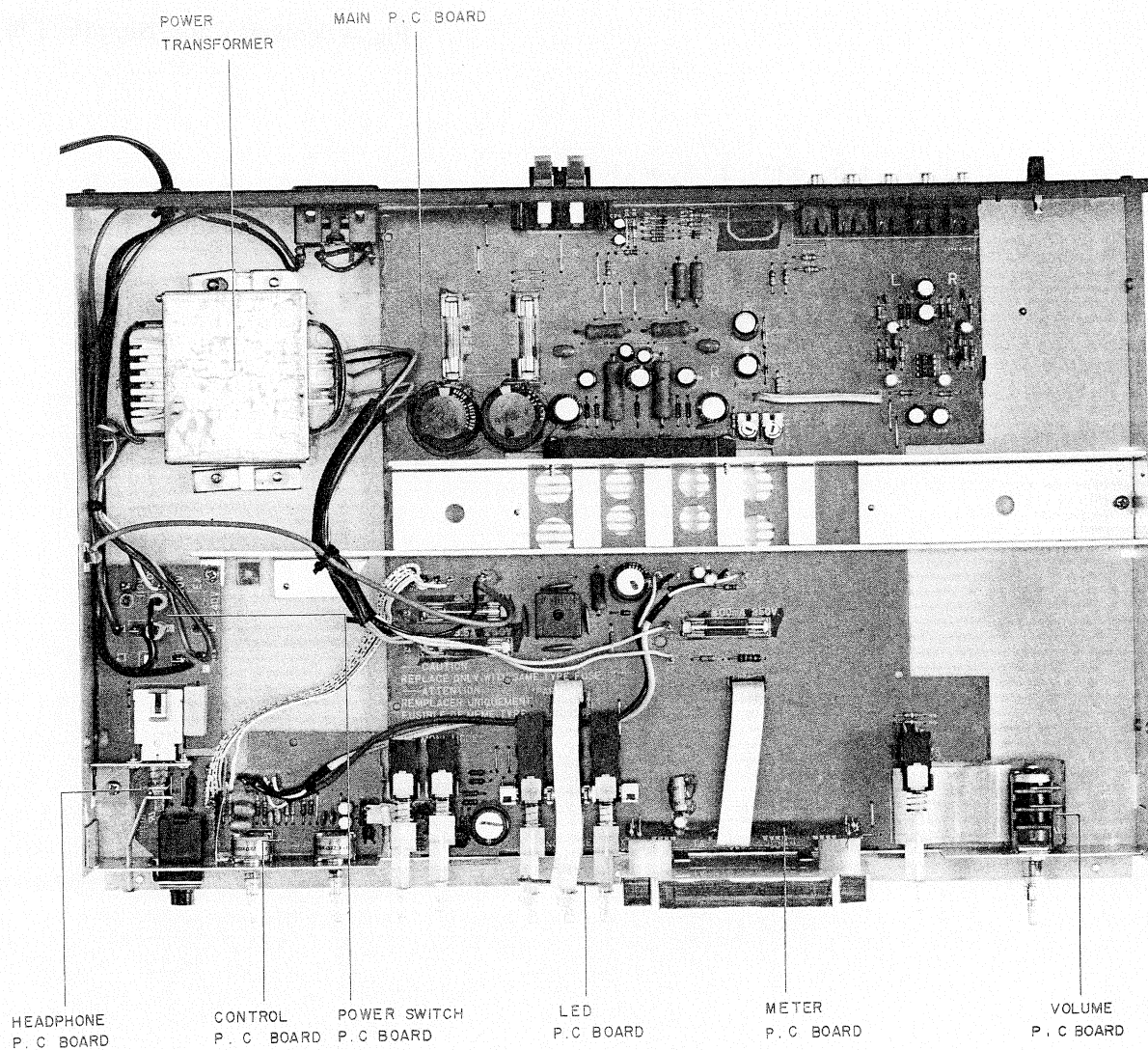
Fig. 3 Top view
