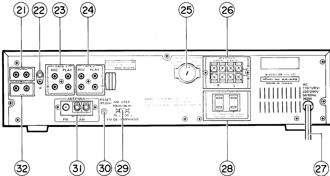
Fig. 3-2 Rear View
