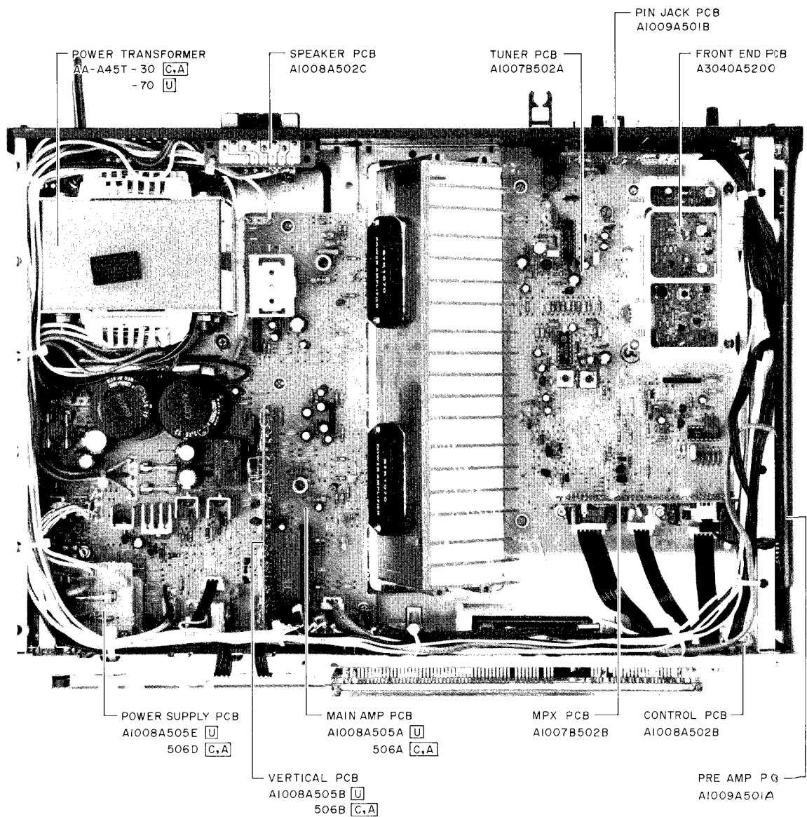
Fig. 4-2 Top View
