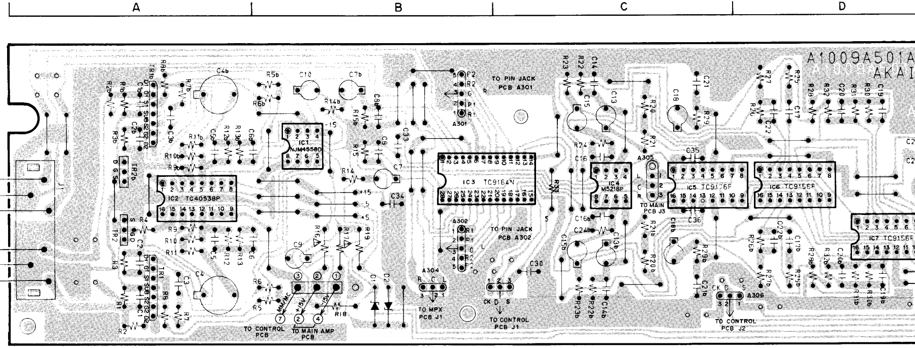
PRE AMP PCB A1009A501A
