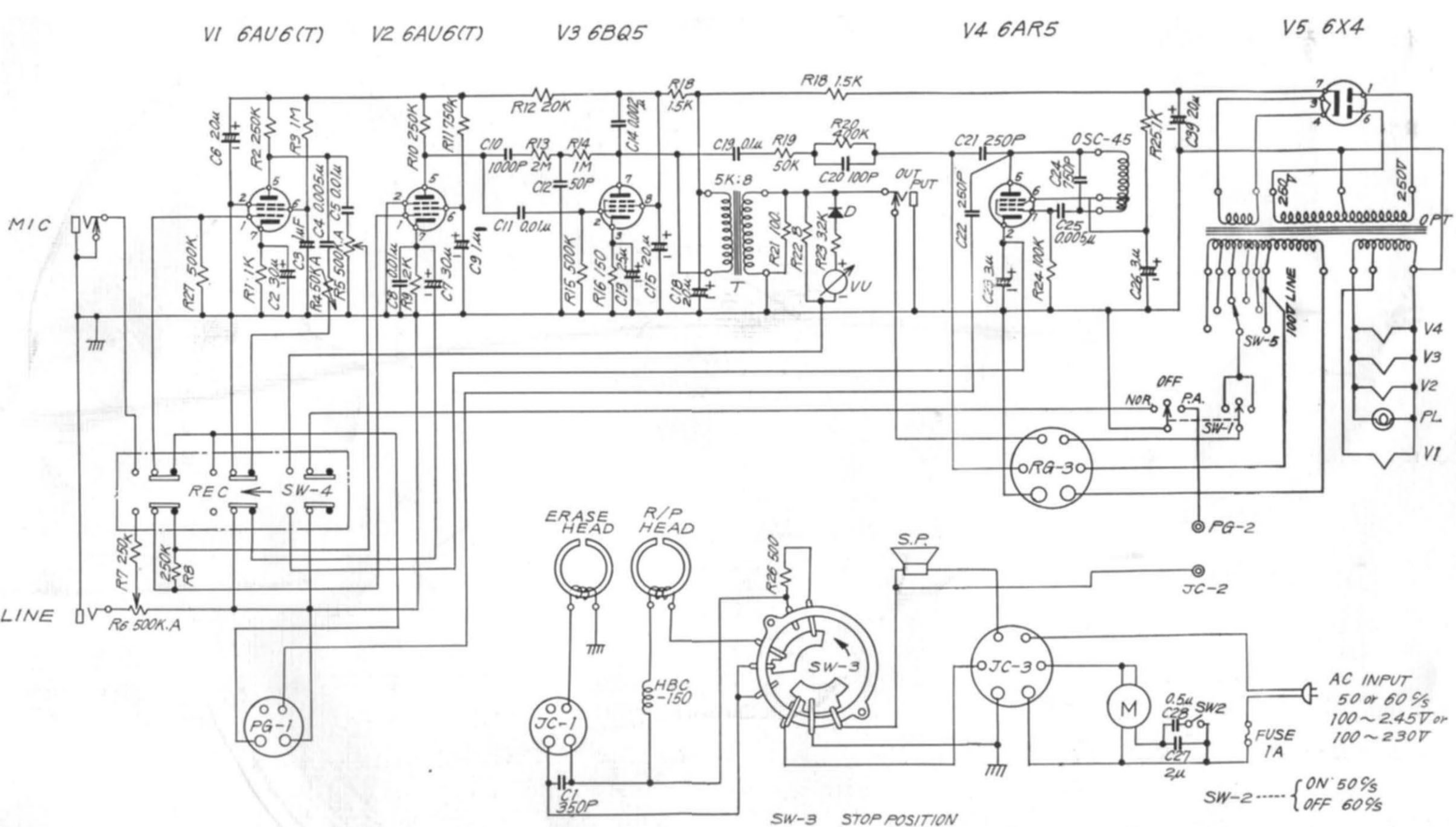
Magnetophone a bande AKAI Mod 910 (tape Recorder Reel-to-reel)
