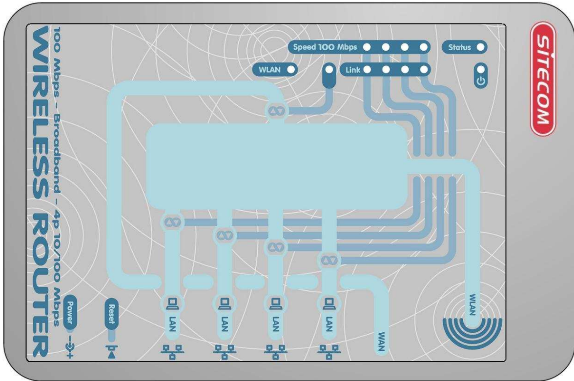
Figure 2-1 Front LEDs
